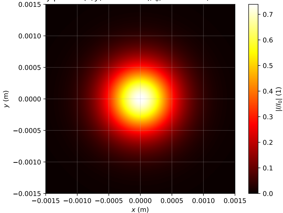
Intensity profile I(x, y, z = 3.423m)/I_0 , \text{Pin}=0.7\text{Pcr} , artificial time
